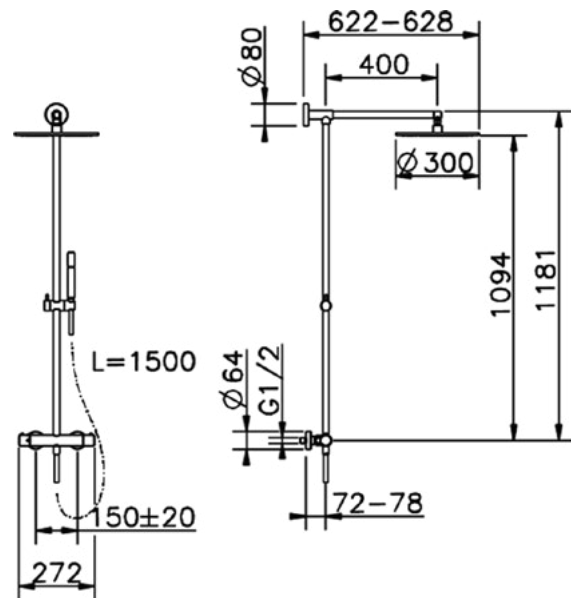
SM C78010 CombiDoccia Termostatico Thermo CombiShower CombiDouche Thermo
