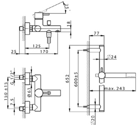
SM 000060 Completo Monocomando Vasca Bath/S. Mixer Set Ensemble Mitigeur Bain/D.
