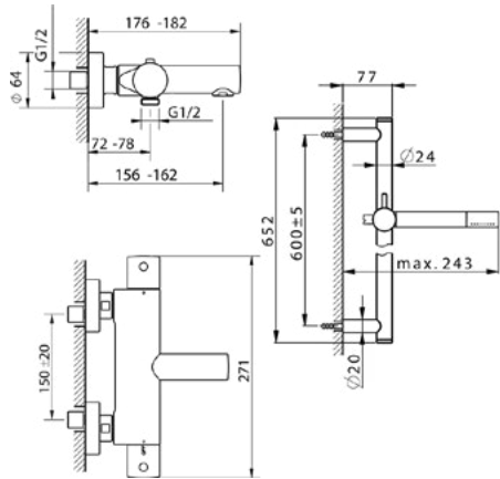
SM S23010 Completo Termostatico Vasca Thermo Bath/S. Set Ensemble Thermo Bain/D.
