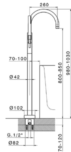
SM 004200 Completo Monocomando Vasca Free-Standing Free-Standing Bath/S. Mixer Set Ensemble Mitigeur Bain/D. Free-Standing
