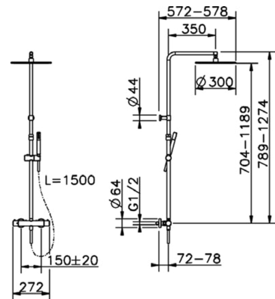
SM C84010 CombiDoccia Termostatico Thermo CombiShower CombiDouche Thermo
